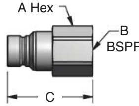
Male Quick Disconnect
