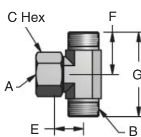
FS.40. Branch Tee
