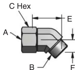
FS.30. Swivel Nut 45° Elbow
